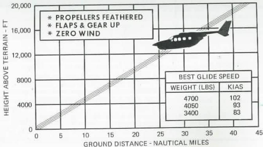
Figure 3-4. Maximum Glide
