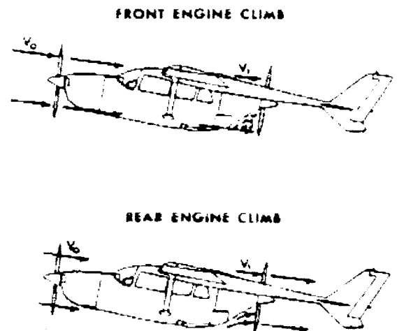
Fig. 1 — Propeller inflow and slipstream effects in single-engine climb
