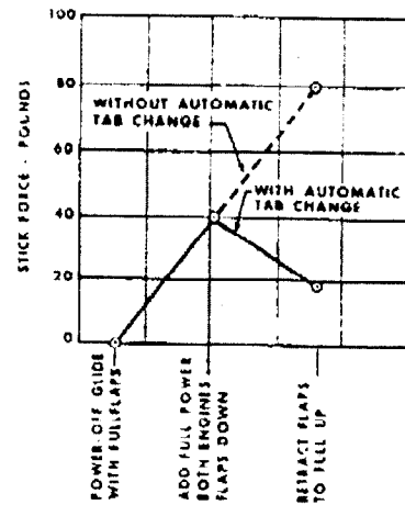
Fig. 3 - Longitudinal trim changes in balked landing go-around
