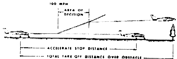
Fig. 5 - Single engine take-off - conventional twin
