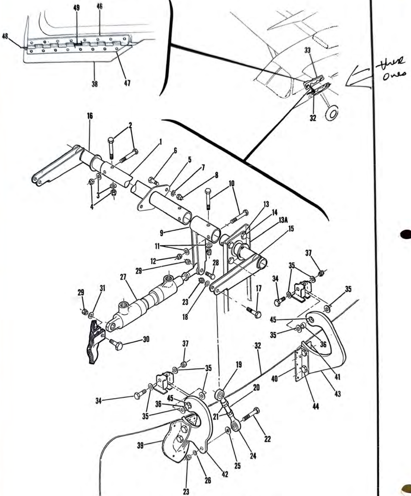
Figure 49. Main Gear Strut Door Linkage Installation
