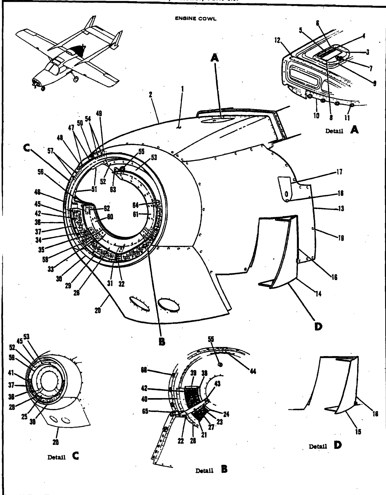
Figure 83. Aft Engine Cowl Installation
